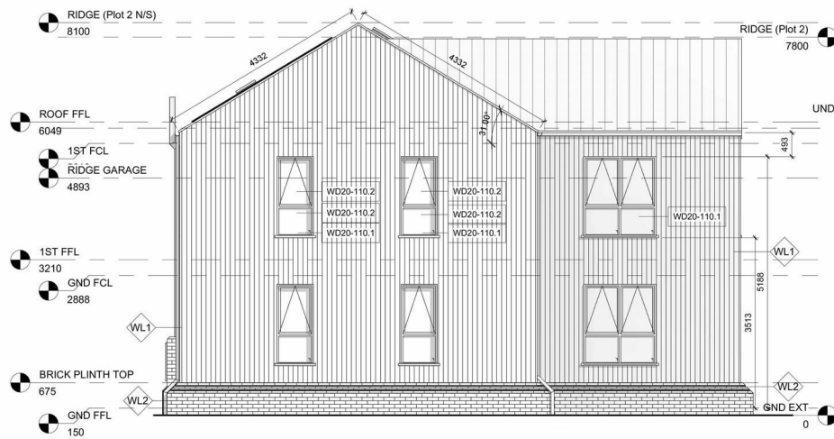
2 PLOT 2 SOUTH 1 : 50
